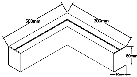
HL 6-1635A/300:300x300x60x80mm
